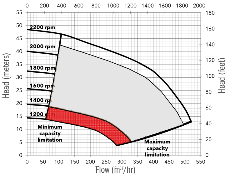
Performance Curve
